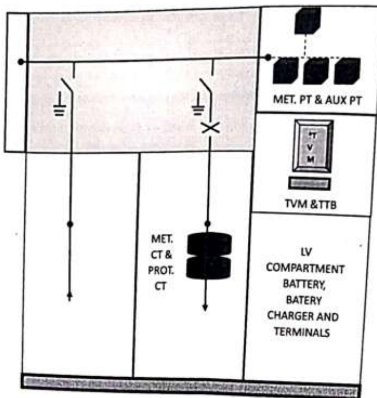
Extensible SF6 insulated panel with metering unit:
